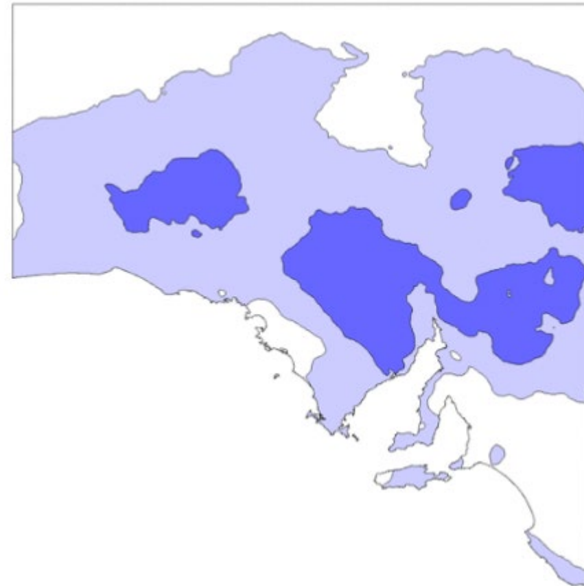
Spring rainfall deciles (Sep-Nov)
