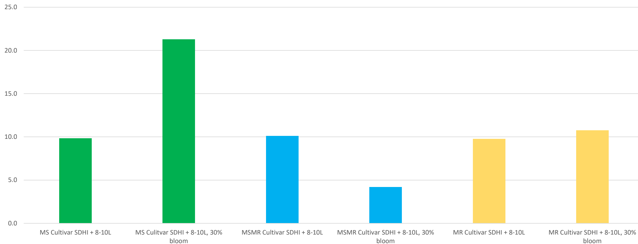
% Yield Increase over Control 2022 Cummins Fungicide Trial
