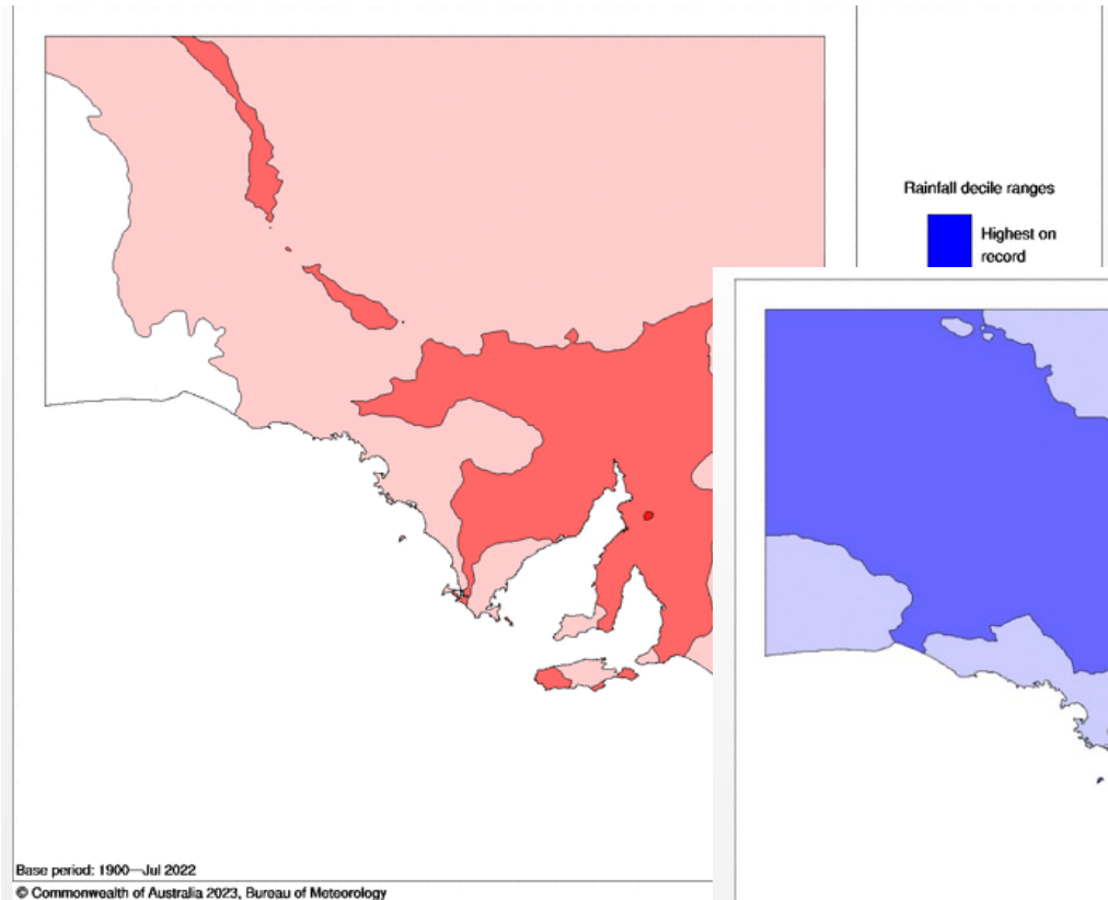
July 2022 rainfall deciles
