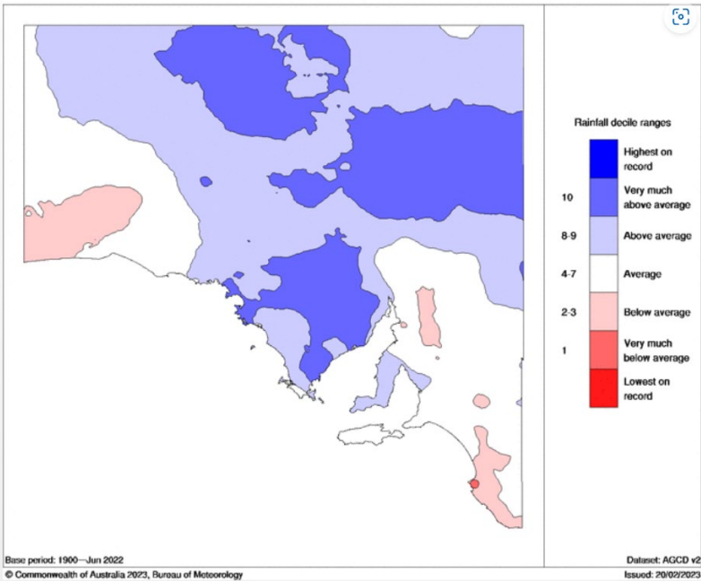
Jan-Jun 2022 rainfall deciles
